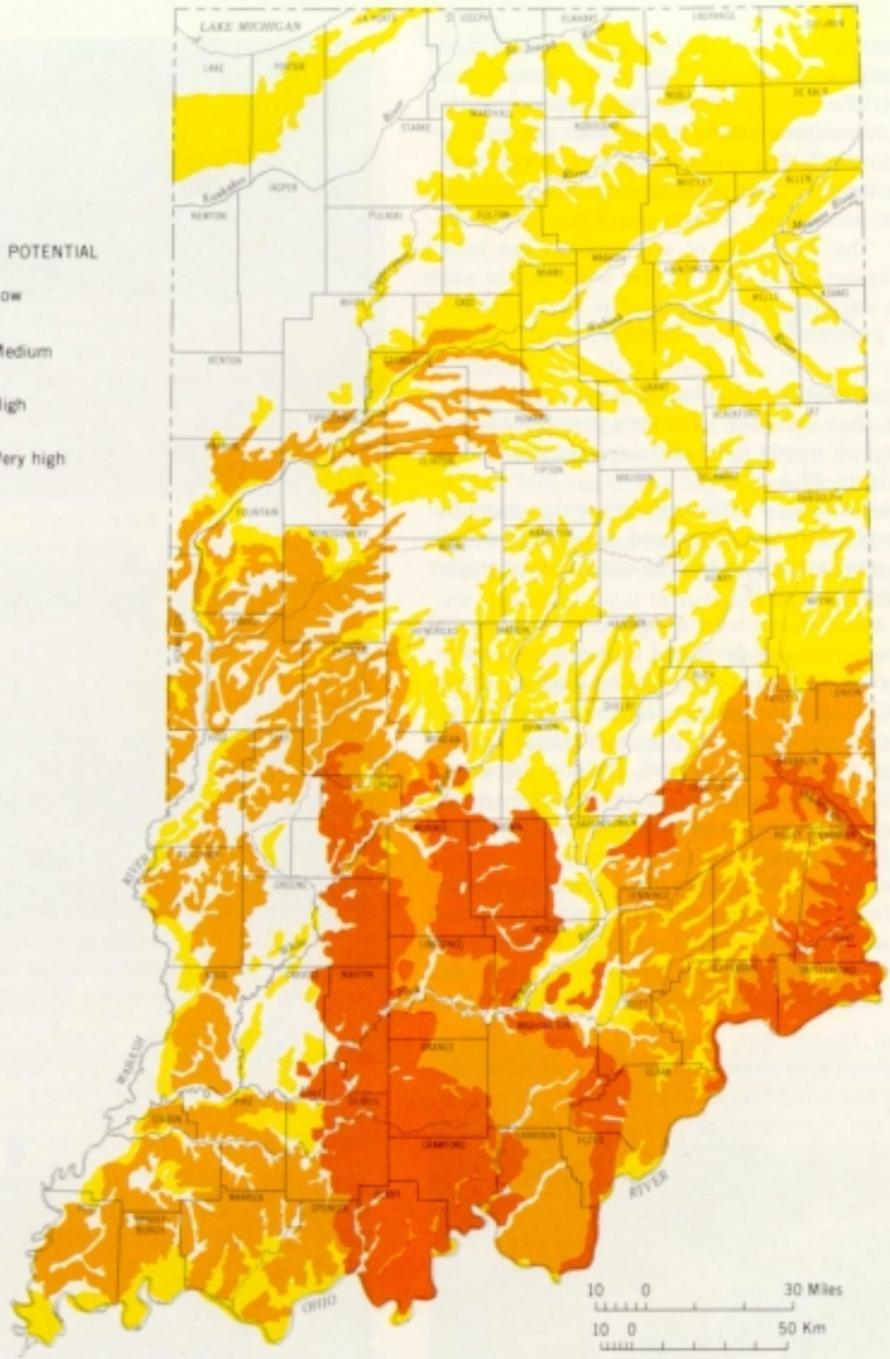
Figure 43 Map showing soil erosion potential of Indiana soil associations.
