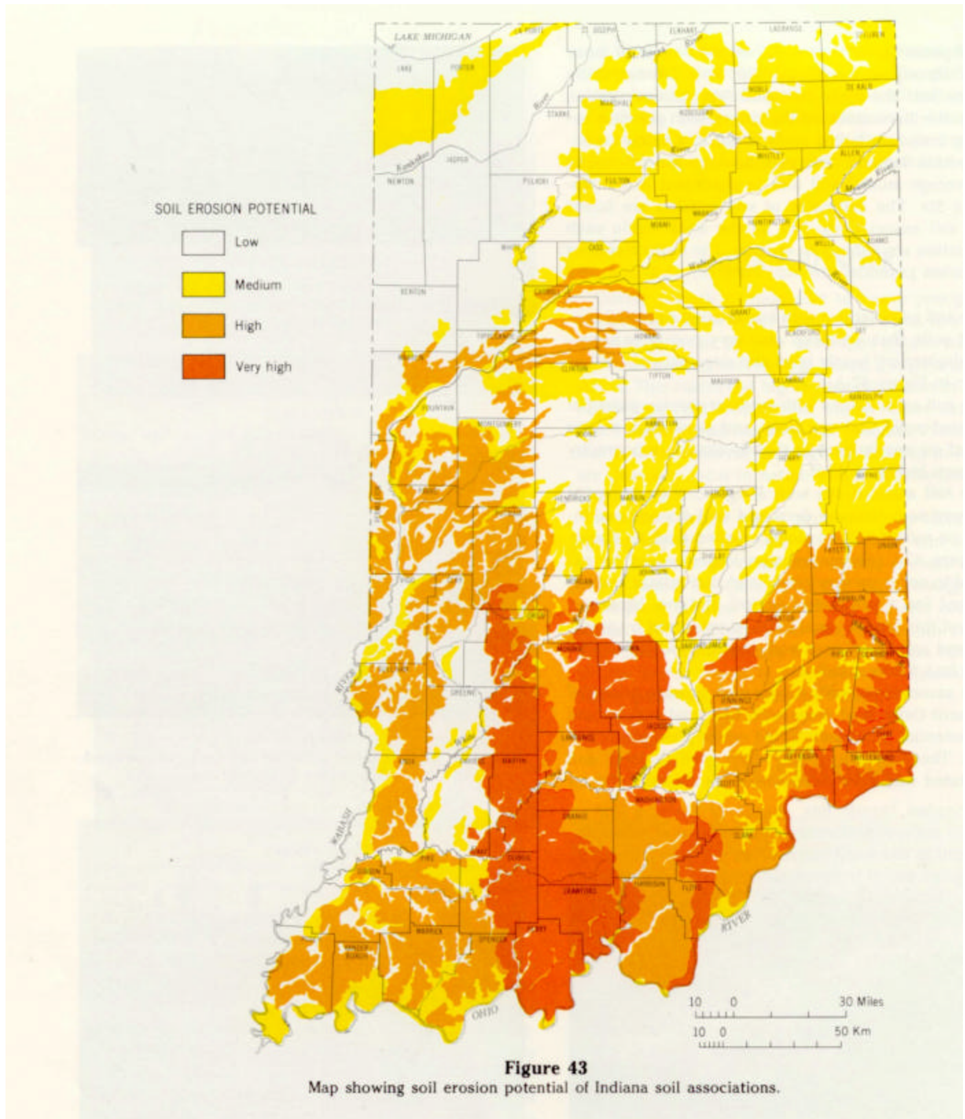
FIGURE 2-3 EROSION POTENTIAL *
