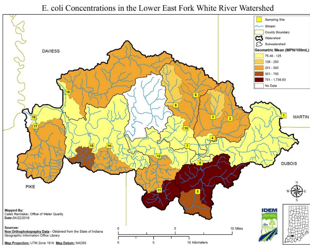
Figure 6: E. coli concentrations based on 5-week geometric mean (MPN/100mL) and sampling site drainage areas for 2017-2018. Values over 125 MPN/100mL are not meeting the current WQS for E. coli .
