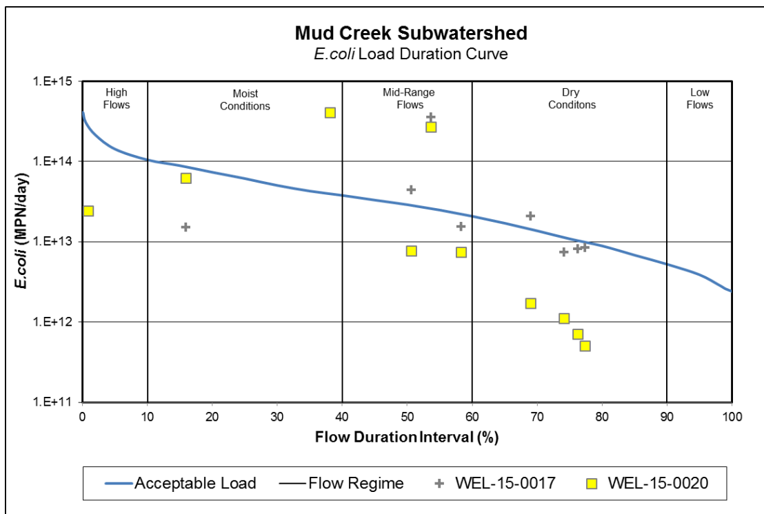
Figure 67: E. coli Load Duration Curve for Mud Creek Subwatershed
