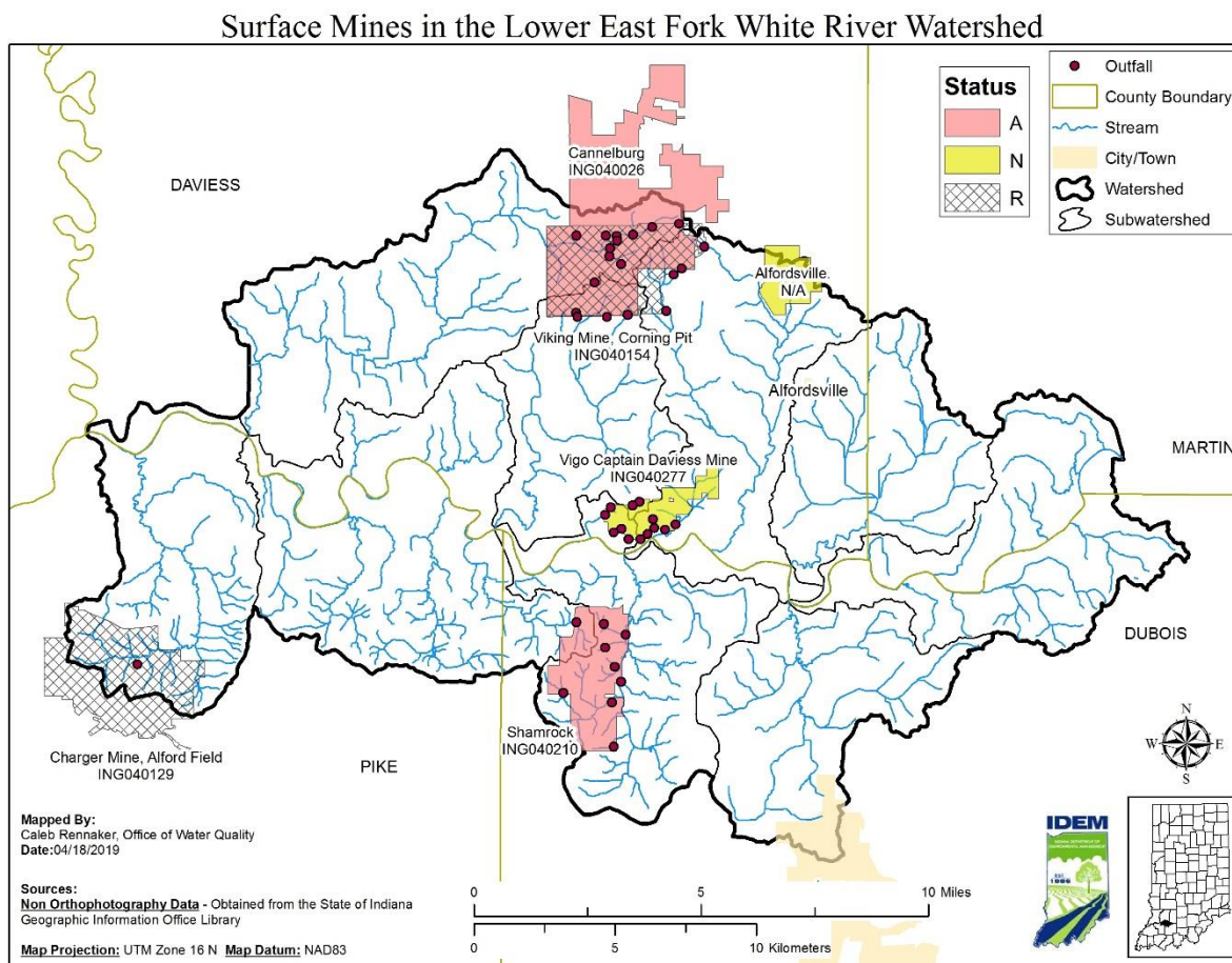
Figure 24: Surface mines in the Lower East Fork White River watershed. Permit status indicated by the following letters: A – active; N – new permit bonded (no overburden removal or coal extracted); R - overburden removal and coal extraction complete.
