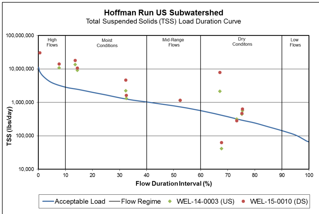
Figure 32: Total Suspended Solids Load Duration Curve for Hoffman Run Subwatershed for Upstream (US) and Downstream (DS) sampling locations.
