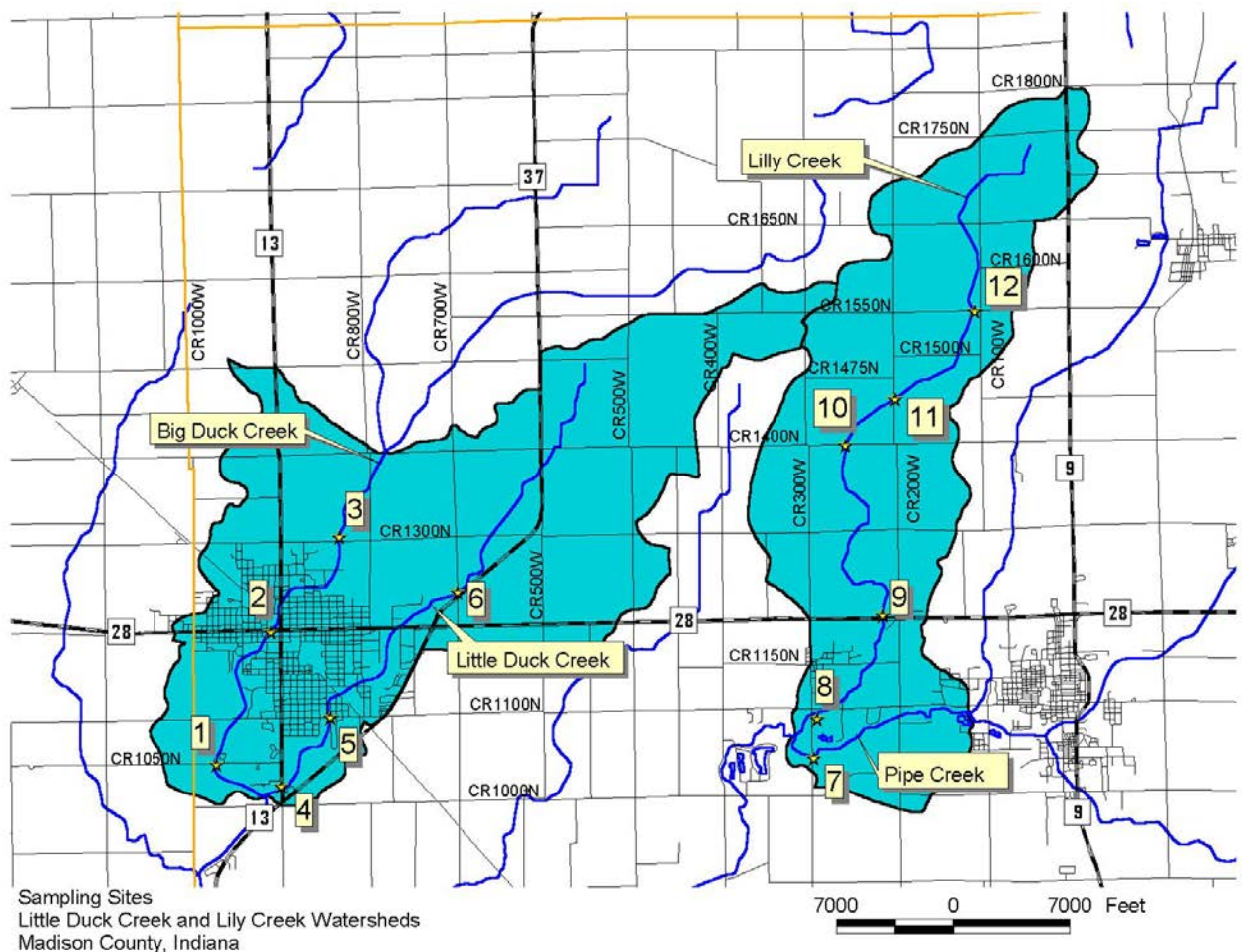
Figure 6 – Sampling Sites.
