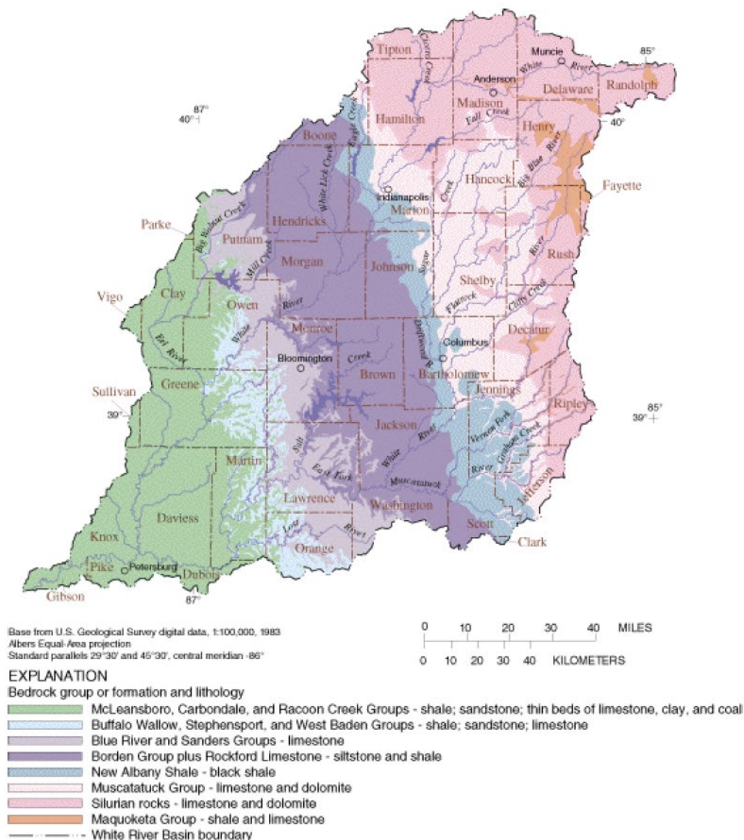
Figure 4 – Bedrock Geology.
