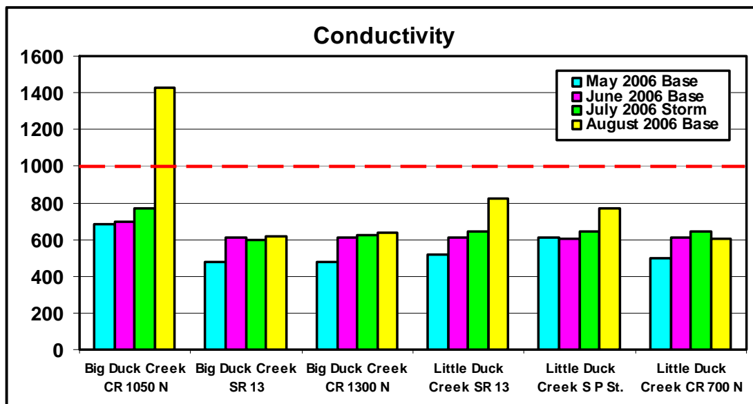
Figure 10. Conductivity measurements for the Little Duck Creek Watershed stream sites for 2006. The low end of the state standard maximum for conductivity is 1000 \mu mhos, which is represented by the dashed line.
