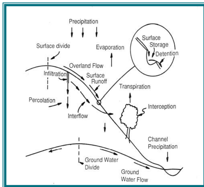
Exhibit 1: The Hydrologic Cycle
