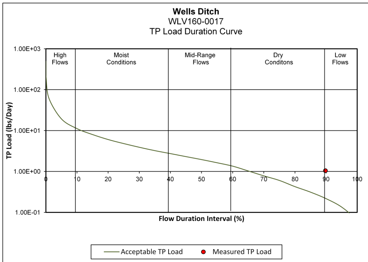
Figure 47. Total Phosphorus Load Duration Curve at Wells Ditch in Headwaters of Big Raccoon Creek subwatershed
