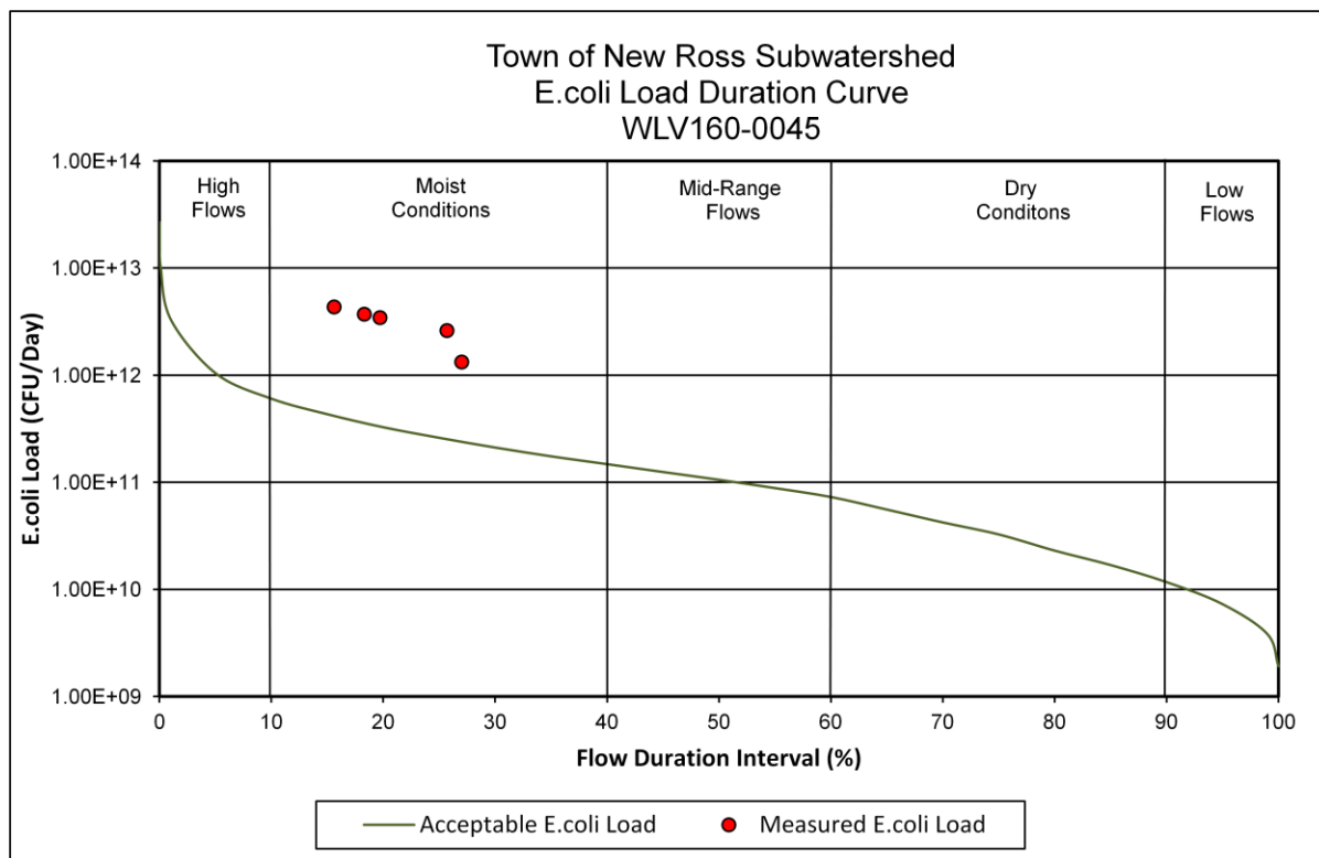
Figure 29. Load Duration Curve in Town of New Ross Subwatershed
