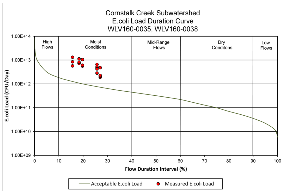
Figure 35. Load Duration Curve for Cornstalk Creek Subwatershed
