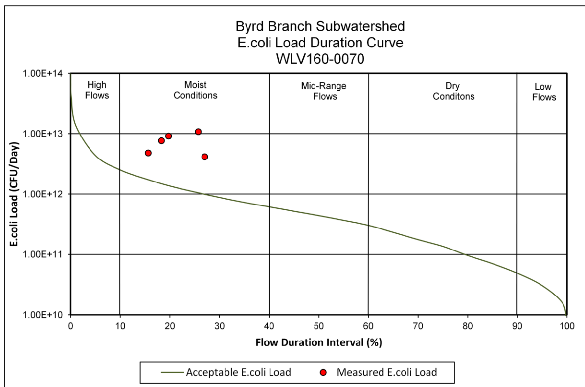
Figure 44. Load Duration Curve in Byrd Branch Subwatershed
