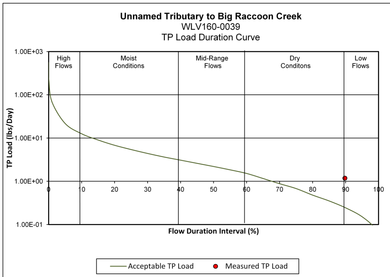
Figure 50. Total Phosphorus Load Duration Curve for the Unnamed Tributary to Big Raccoon Creek
