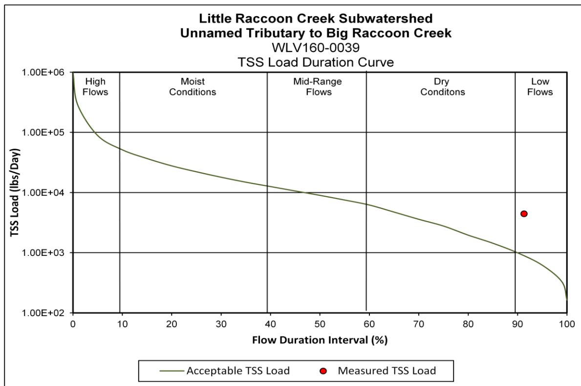
Figure 53. Total Suspended Solids Load Duration Curve for the Unnamed Tributary to Big Raccoon Creek
