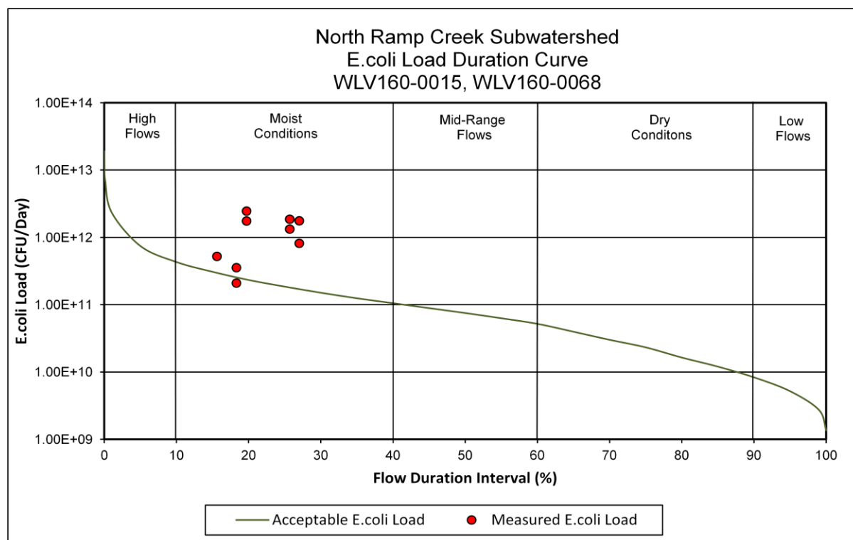
Figure 38. Load Duration Curve for North Ramp Creek Subwatershed
