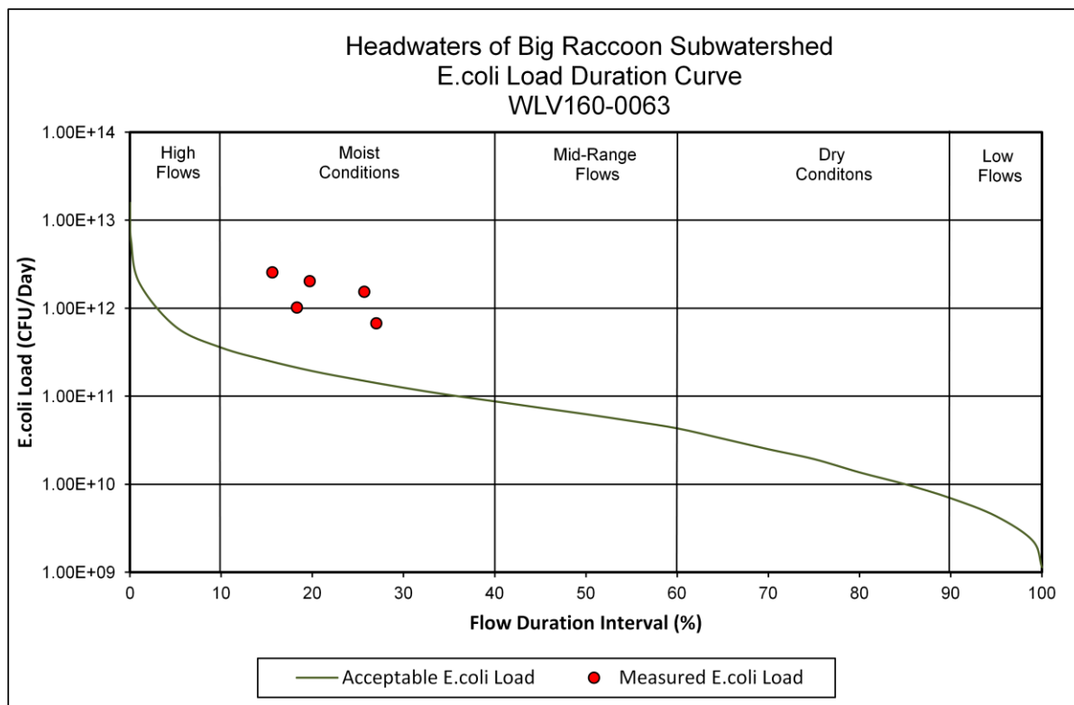
Figure 26. Load Duration Curve in the Headwaters of Big Raccoon Creek Subwatershed
