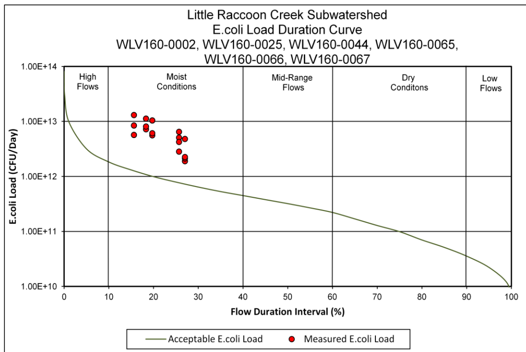
Figure 41. Load Duration Curve for the Little Raccoon Creek Subwatershed
